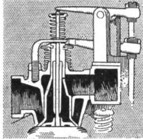
Franklin Valves.
